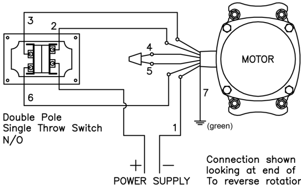
Switch Schematic (Double Pole, Single-Throw momentary-contact normally open)
